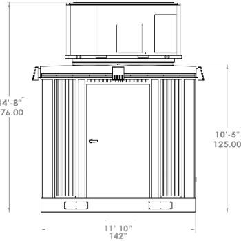
ELEVATION VIEW
