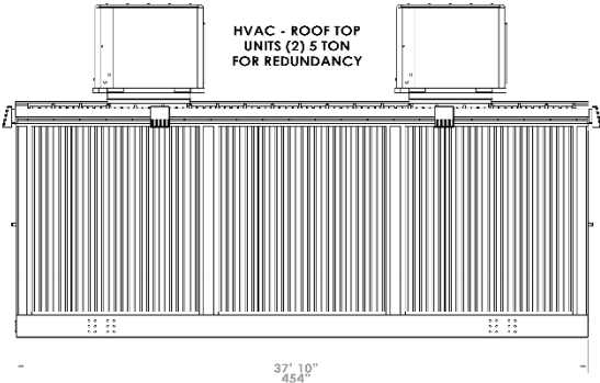
ELEVATION VIEW
